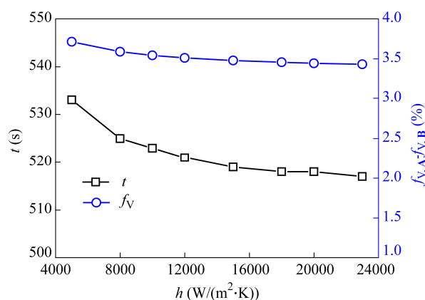
Fig. 7 Curve of mold-opening time and rubber cure uniformity versus the convective heat transfer coefficient of heating boundary
